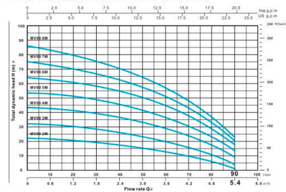
PERFORMANCE DATA AT n= 2850 min -1
